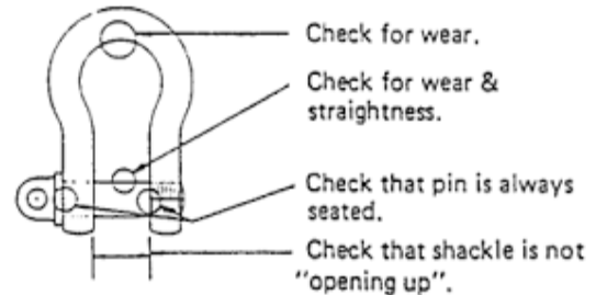
Figure 7. Areas of Shackle Wear
