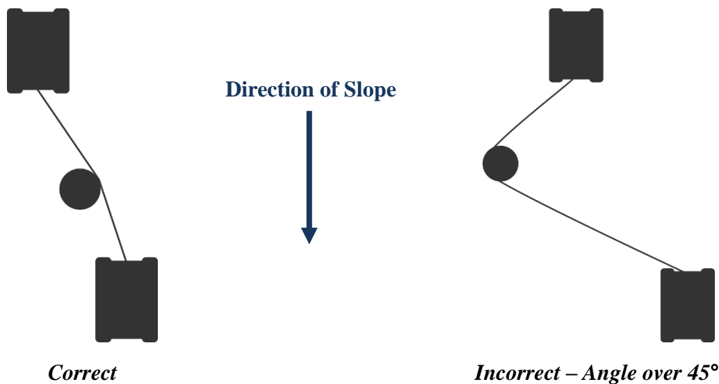
Figure 1. Wire rope side wash
