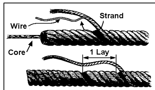
Figure 4. Strand and Lay of Wire Rope
