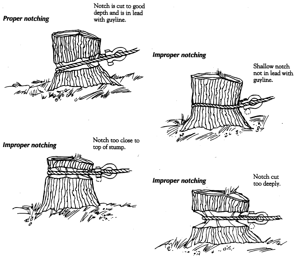
Figure 5. Correct Anchor Notching
